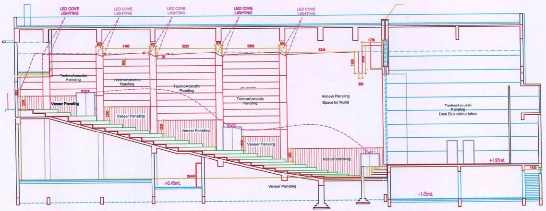
SECTIONAL ELEVATION
