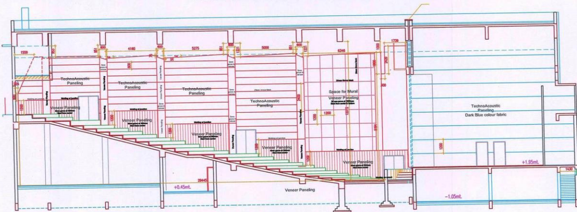
SECTIONAL ELEVATION
