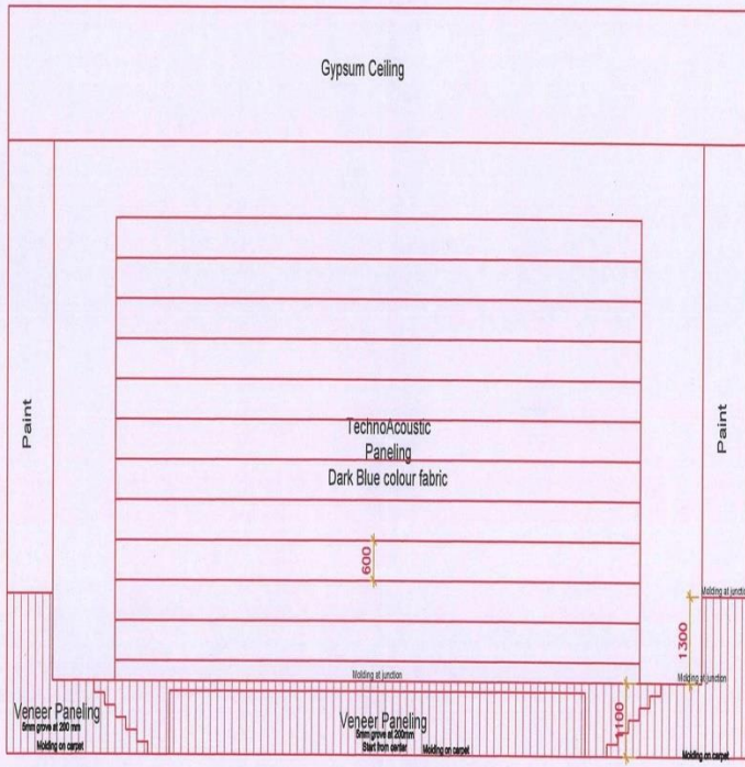
AUDITORIUM ACOUSTICAL TREATMENT
